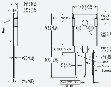
TO-247 3-Lead
