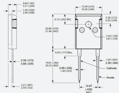
TO-247 2-Lead
